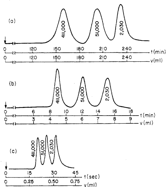
Figure 5. Chromatographic experiment time influenced by particle size: polystyrene standards. (a) Chromatogram synthesized from the data of ref 25. Conditions: d_{p\text{max}} = 120 \mu of GPC 10-2000, 10-1250, 10-700, 10-370, 10-240. Five-column series, L = 20 ft, i.d. = 0.305 in., flow rate 1.0 ml/min; toluene eluent. (b) Conditions: d_{p\text{max}} = 44 \mu ; GPC 10-700, 10-350, 10-125; three columns, L = 150 cm, i.d. = 2.6 mm; F = 0.5 ml/min; tetrahydrofuran eluent. 22 (c) Conditions: d_{p\text{max}} = 6 \mu , Zorbax porous silica microspheres; one column, L = 50 cm, i.d. = 2.0 mm; flow rate 1.0 ml/min; tetrahydrofuran eluent. Redrawn from ref 8 with permission of the copyright owner.
