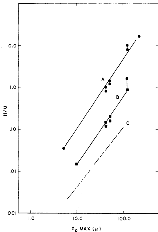
Figure 4. Plate height as a function of d_{p\text{max}} for rigid porous packings. Curve A: H_{\text{poly}}/U for narrow polystyrenes, K_{\text{GPC}} = 0.5 \pm 0.1 , calculated from ref 8, 22-26. Curve B: H/U for monomeric solutes, K_{\text{GPC}} \approx 1.0 , from ref 8, 13, 22-26. Curve C: indicated lower limit of H/U , from ref 8.
